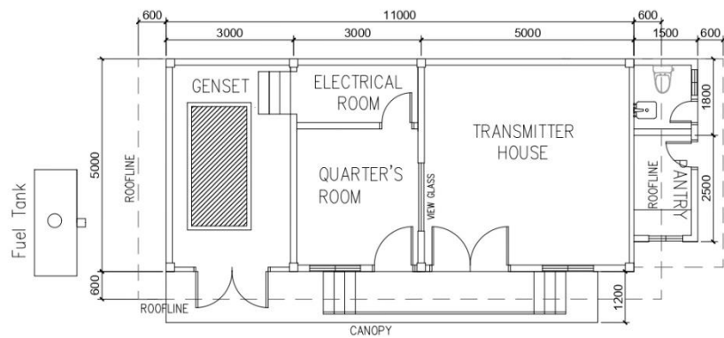
FLOOR PLAN (TRANSMITTER BLDG.)
