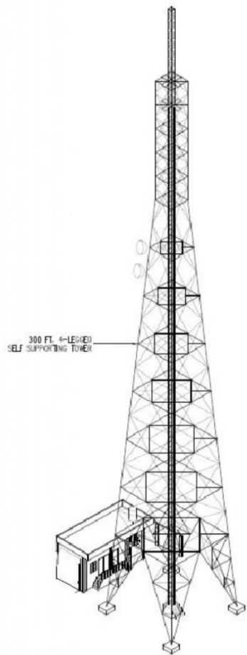
300FT. 4-LEGGED TOWER
