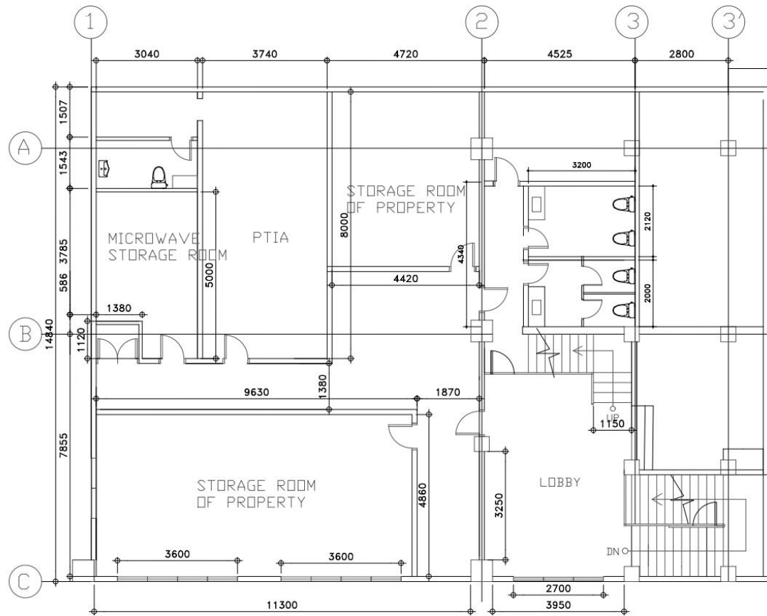
EXISTING PLAN SECOND FLOOR
