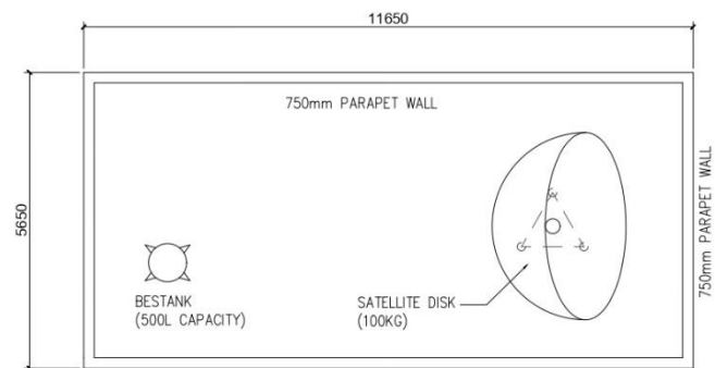
ROOF DECK PLAN
