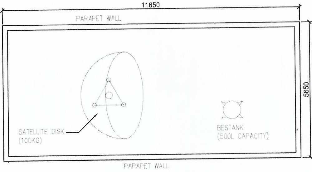
ROOF DECK PLAN
