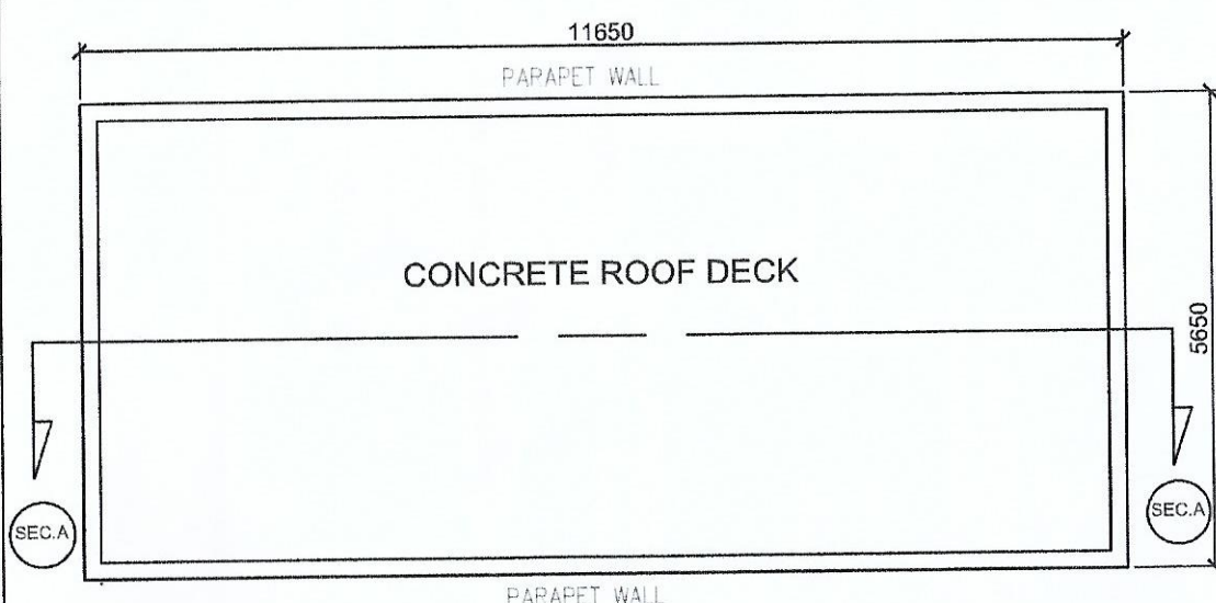
TOP VIEW PLAN
